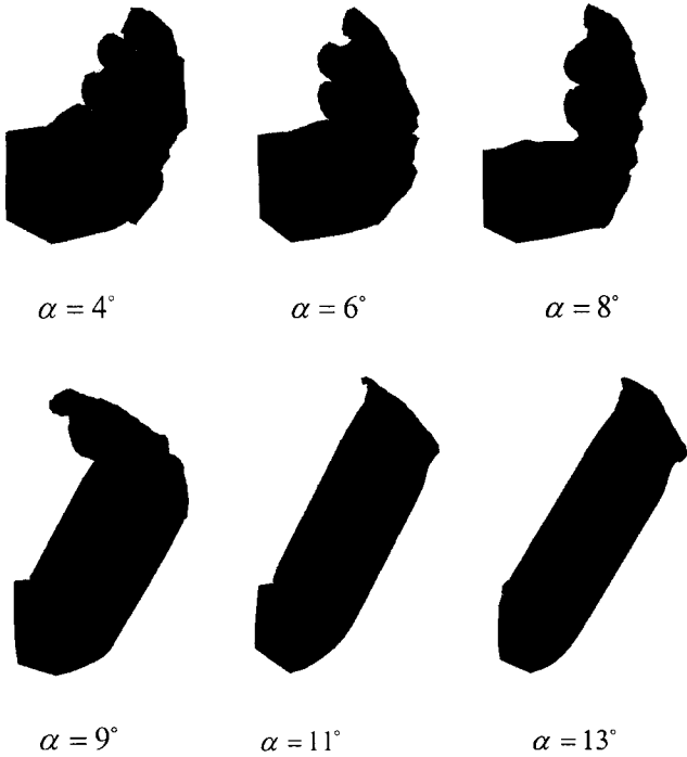
Figure 2 Deformed shapes with different crash angles
