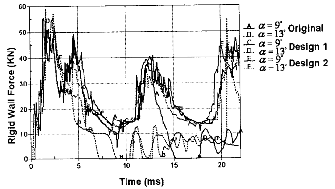
Figure 20 Comparisons of rigid wall forces for different Designs
