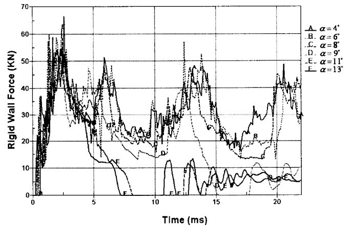
Figure 3 Crash force history with different crash angles
