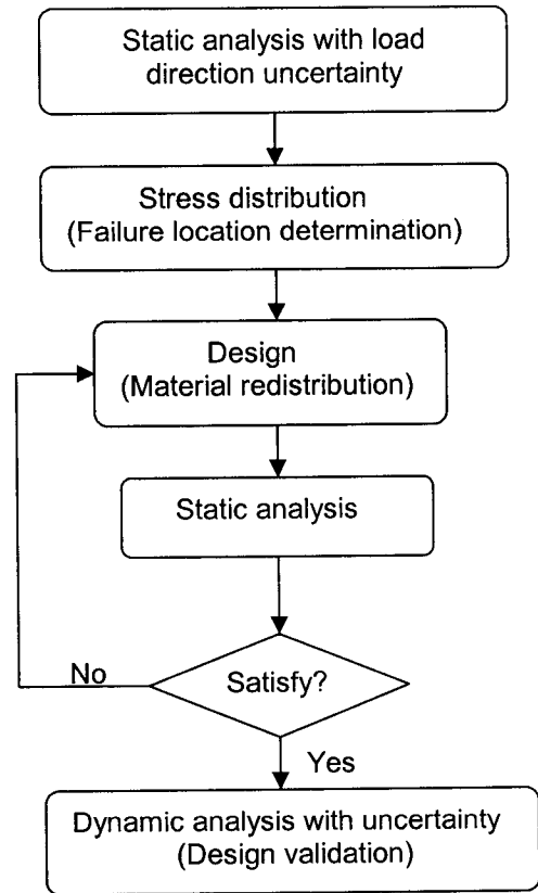
Figure 18 Design procedure
