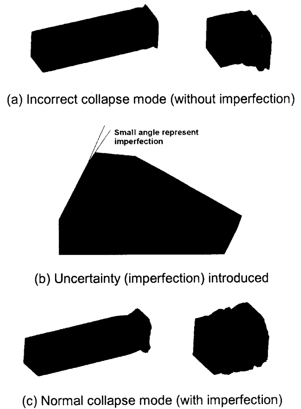
Figure 6 Influence of modeling uncertainty
