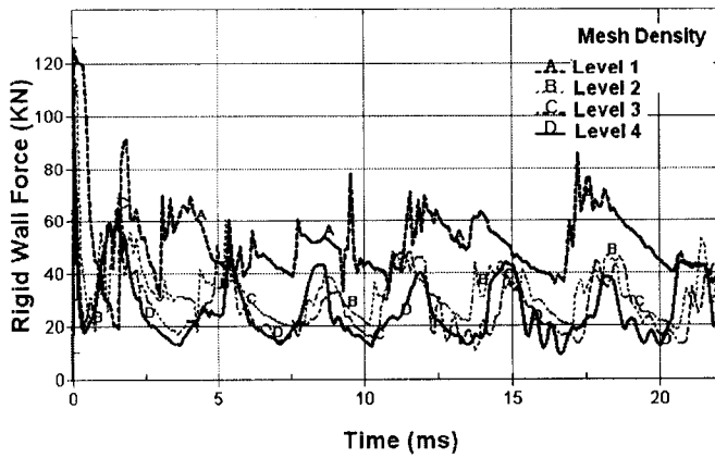
Figure 8 Crash force history for different mesh densities
