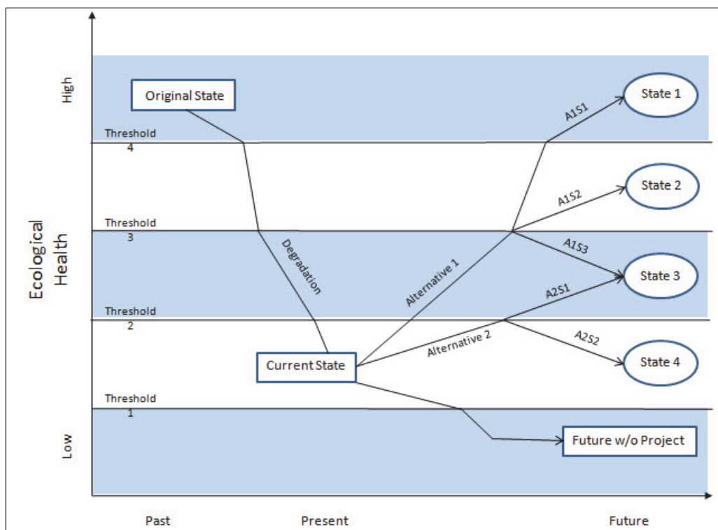
Figure 4. Various ecological trajectories and alternative future states of an impaired site.
