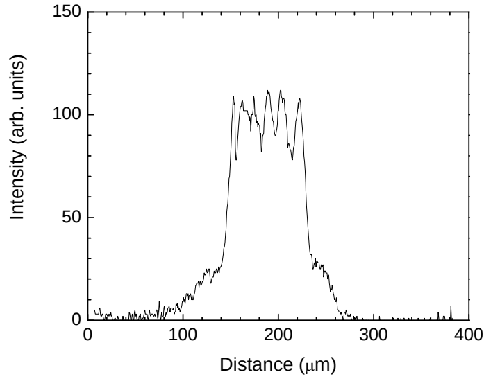
Figure 23: The near-field image of the 2.3 \mu\text{m} diode lasers.
