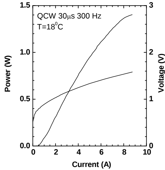
Figure 25: Quasi-CW power (30 μs pulse width, 300 Hz repetition rate) and voltage–current characteristics of 2-mm lasers obtained at a heat sink temperature of 18°C.
