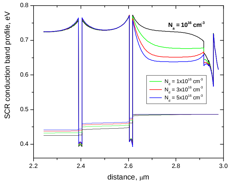
Figure 11: Conduction band profiles of SCR for different levels of the SCR3 layer doping. Profile with N_a = 10^{16} \text{ cm}^{-3} represents the unintentionally p-doped layer.
