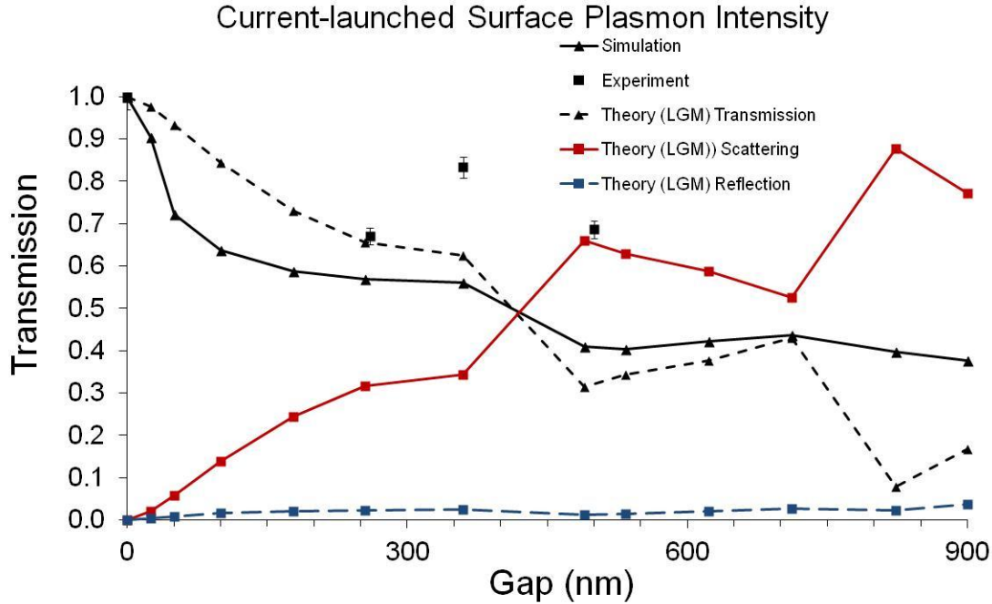
Fig. 24: Surface plasmon transmission across a transverse gap as a function of the gap width and our experimental results. The transmission is relative value of S_z , averaged vertically as described in Fig. 23, but normalized to a value of 1.0 for the averaged Poynting vector 16.6 \mu\text{m} from the current source when there is no gap. Results are also shown using the “tight-binding”-like theory of ref. [37] for the total SPP transmission, losses due to scattering of the electromagnetic energy from the SPPs into the vacuum at the gap, and the back-reflection of SPPs from the gap.
