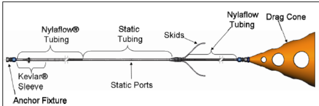
Figure 3 Trailing Cone System with Skids
