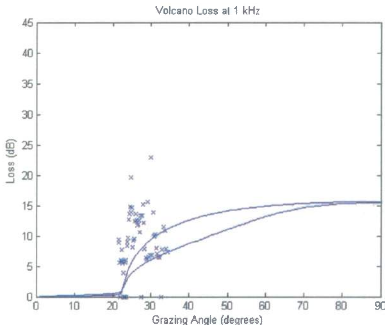
Figure A1: Mud Volcano Bottom Loss Measurements at 1 kHz. Theoretical values are represented by solid lines. The bottom curve assumes that an acoustically hard layer covers the mud volcano.
