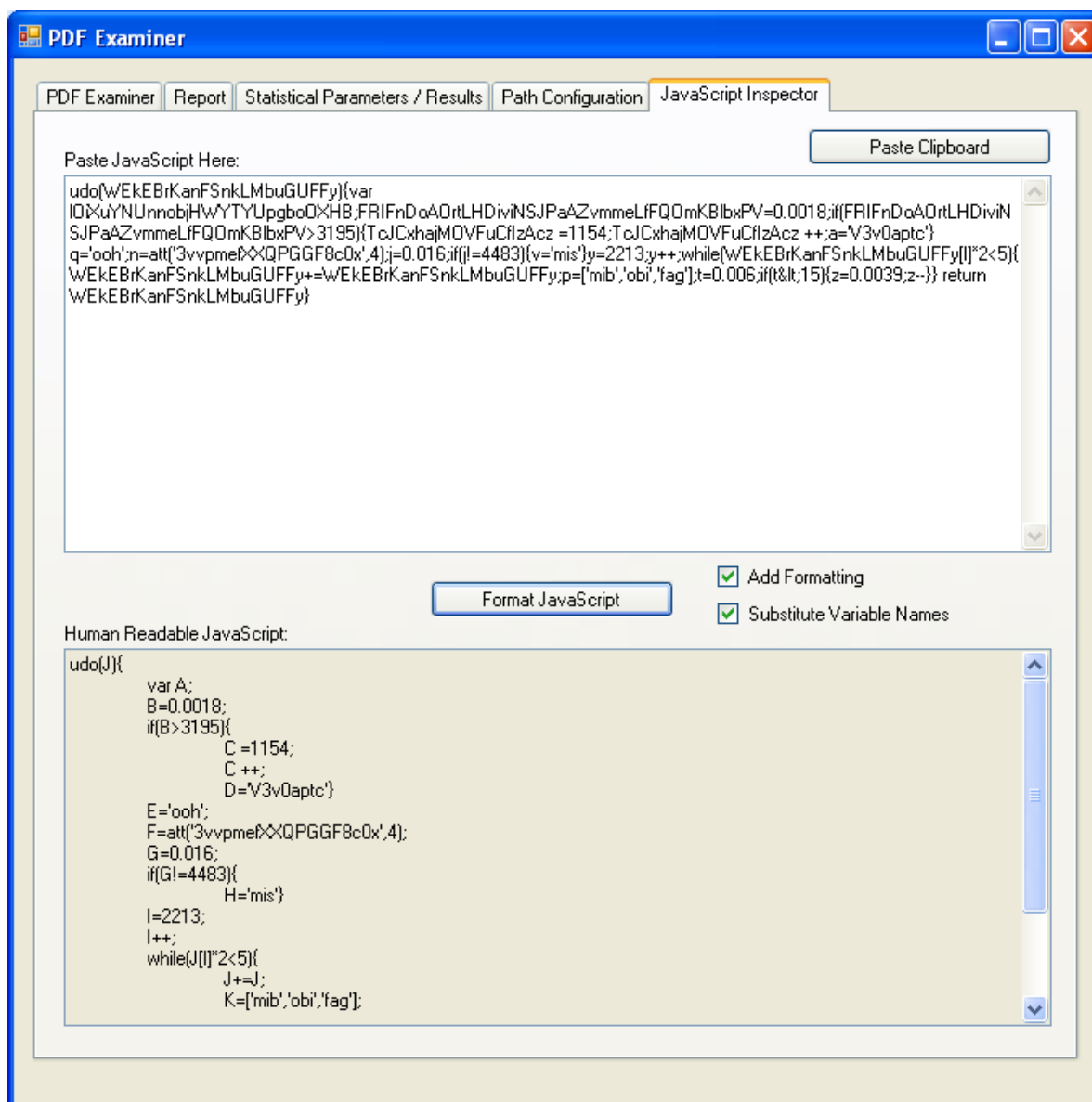
Figure 69. JavaScript re-formatter
