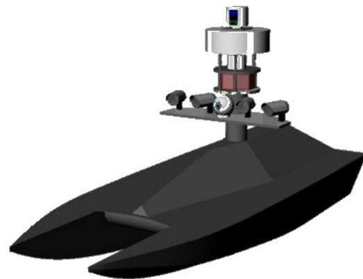
Figure 8: UV Sentry HySuCat concept.
