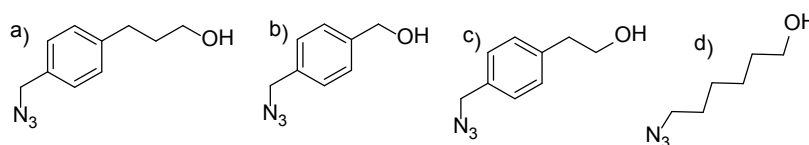
Figure 1. Azido precursors (a-d)
