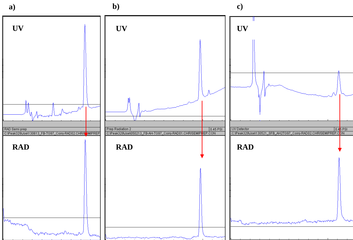
Figure 2. HPLC traces: co-injection of [ ^{18}\text{F} ]SFB conjugated lead analogues with their complementary non-radioactive standards. Top traces are UV channel at 254 nm of the non-radioactive standard and the bottom traces are the RAD channel of the [ ^{18}\text{F} ]FB-TG97 analogues a) [ ^{18}\text{F} ]FB-TG97 b) [ ^{18}\text{F} ]FB-AH-TG97 c) [ ^{18}\text{F} ]FB-AH2-TG97
