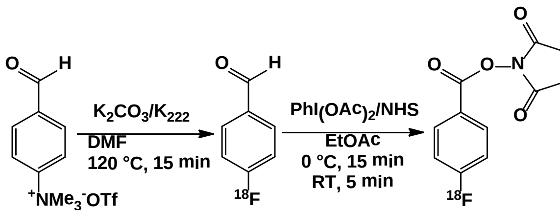
Scheme 1. [^{18}\text{F}] N-succinimidyl-4-fluorobenzoate ( [^{18}\text{F}] SFB)
