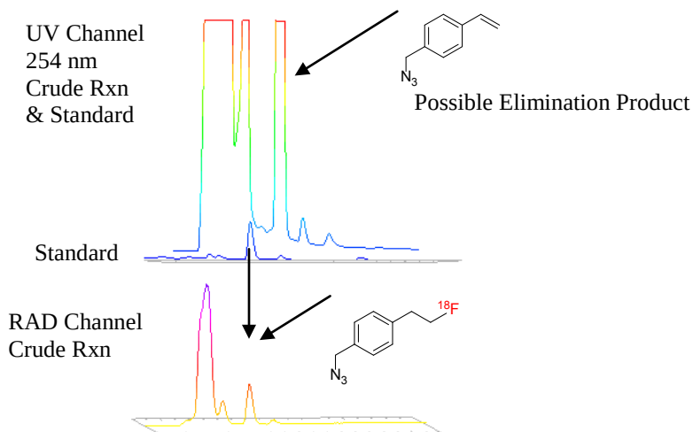
Figure 7. UV/RAD HPLC Precursor 2 ^{18}\text{F} Crude Reaction with overlay with the non-radioactive standard to product confirmation
