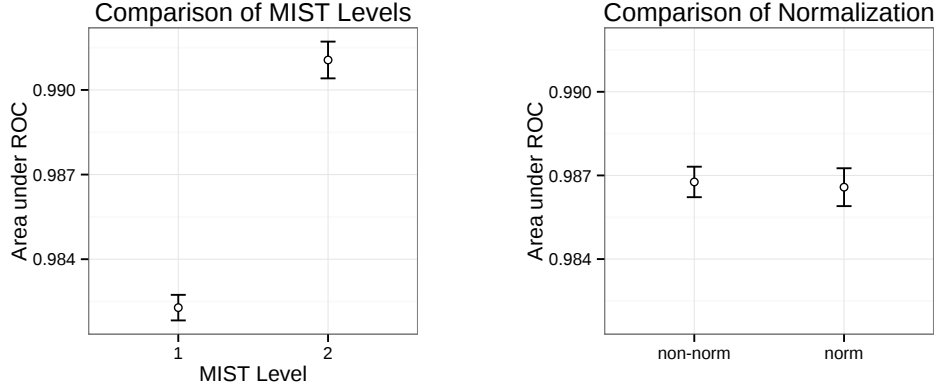
Figure 4.2: Details and chart of area under ROC comparisons of classifier performance by MIST level and normalization with 99.9% confidence intervals
