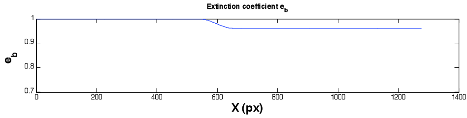
Figure 10: Spatial distribution of the extinction coefficient e_b across the spray for the first scanned beam. Spray centreline is at X=600\text{px}
