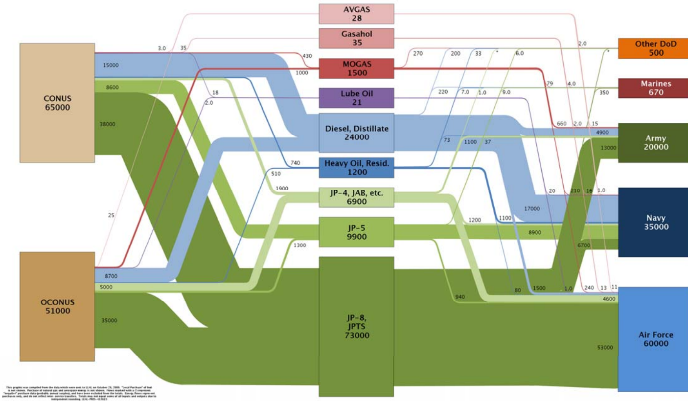
Figure 5. DoD Petroleum Use in 2008, Shown in Thousands of Barrels (From Kaahaaina, 2013, p. 2) Notes. Image created by LLNL from data provided by DLA-E. AVGAS is aviation gasoline; gasahol is gasoline blended with ethanol; MOGAS is motor gasoline; and distillate is F-76.
