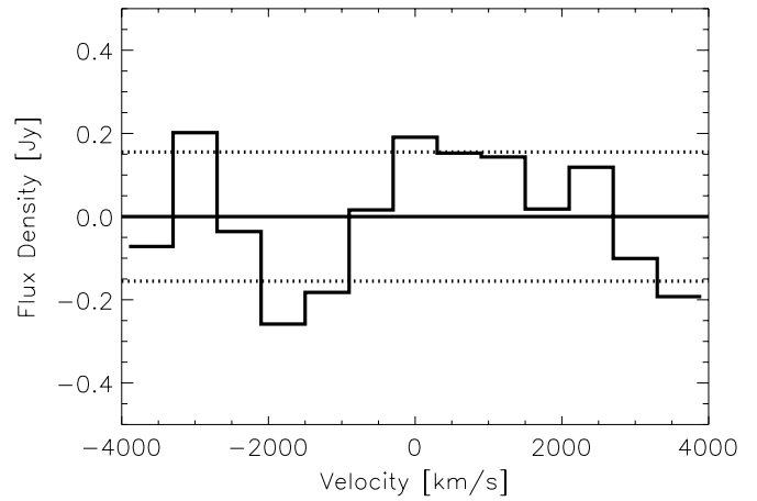
Figure 11. Baseline-subtracted stack of eight transitions with J_{upper} = 34 - 47 , for comparison with the Krolik & Lepp (1989) models. Dashed lines mark the \pm 1\sigma uncertainty.
