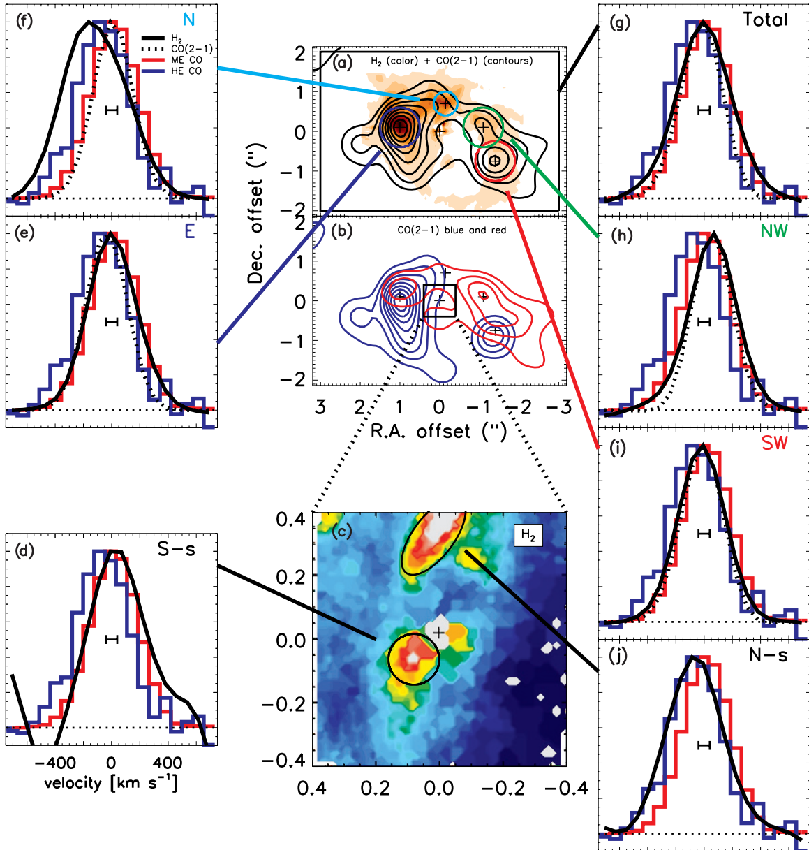
Figure 8. (a) CO(2–1) (contours) and H 2 1–0 S(1) (color) images of the central 4'' × 6'' from Schinnerer et al. (2000) and Müller Sánchez et al. (2009), (b) blue and red components of CO(2–1), with crosses marking the centers of the apertures in panel (a), (c) H 2 1–0 S(1) image of the central 0''.4, (e)–(j) smoothed H 2 1–0 S(1) (black solid) and CO(2–1) (black dashed) profiles from selected apertures in the H 2 ring compared with the ME (red) and HE (blue) composite profiles, and ±40 km s −1 horizontal error bar indicating the calibration uncertainty between the FIR CO and H 2 spectra, (d), (j) smoothed H 2 1–0 S(1) profiles from the northern and southern streamer compared with the ME and HE composite profiles, and ±40 km s −1 horizontal error bar.
