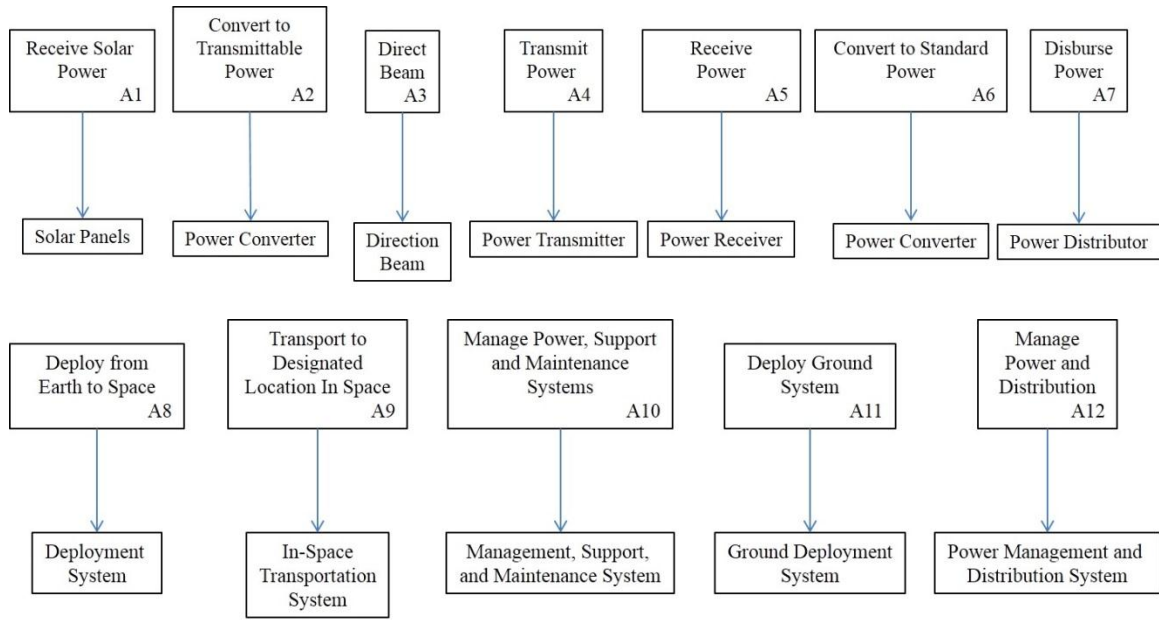
Figure 11. Allocated architecture
