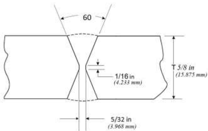
Figure 2 Tandem Wire Weld Joint Geometry
