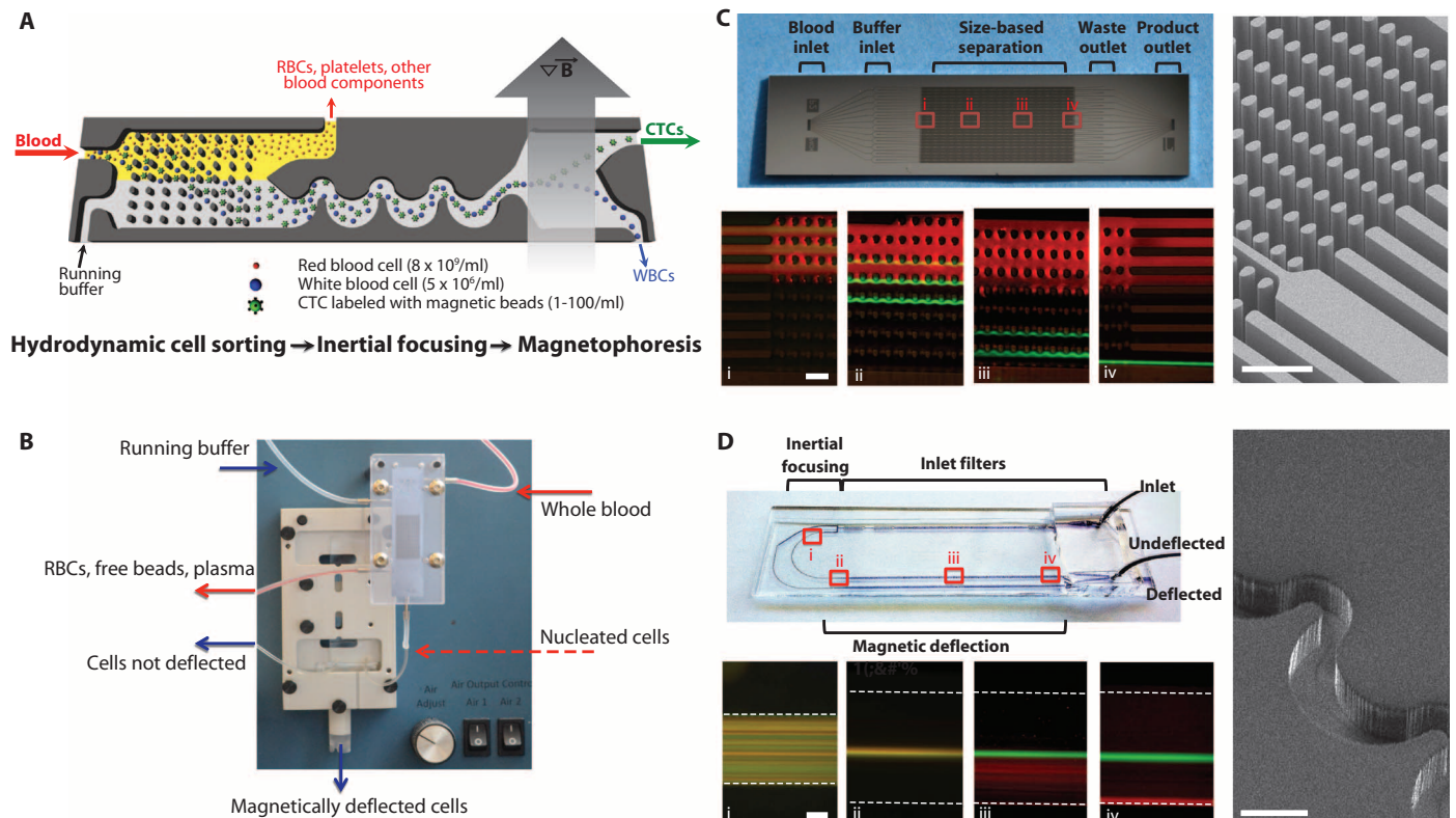
Fig. 1. The CTC-iChip system. (A) Three microfluidic components of the CTC-iChip are shown schematically. Whole blood premixed with immunomagnetic beads and buffer comprises the inputs. The figure demonstrates the positive isolation method; however, the system can be operated in negative depletion mode. (B) Integrated microfluidic system. The debulking array sits in a custom polycarbonate manifold that enables fluidic connections to the inputs, waste line, and second-stage microfluidic channels. The inertial focusing and magnetophoresis chip is placed in an aluminum manifold that houses the quadrupole magnetic circuit. Magnetically deflected cells are collected in a vial. (C) Hydrodynamic size-based sorting. A mixture of 2- \mu\text{m} (red) and 10- \mu\text{m} (green) beads enters the channel (i).
