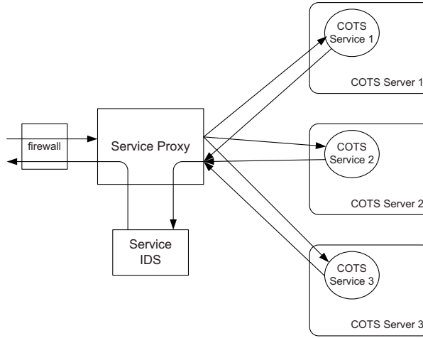
Fig. 1. General Pattern of Intrusion Tolerance Architecture
