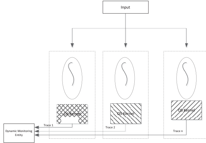
Fig. 2. Architecture for Diversity-based Dynamic Monitoring
