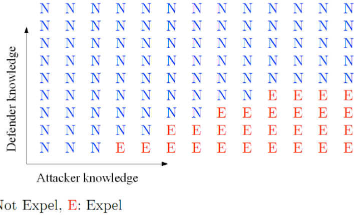
Figure 4: The optimal policy in control-matrix form.
