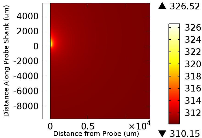
Surface: Temperature (K)
