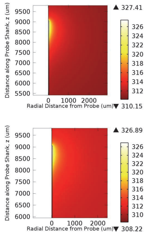
Figure 6a and 6b: 6a: Temperature distribution surrounding the heating probe without modeling the effects of blood perfusion. 6b: Temperature distribution including the effects of blood perfusion.
