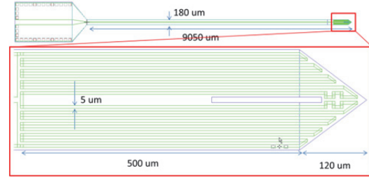
Figure 3: Mask layout for a neural probe containing an ohmic heater being investigated and designed by this work.
