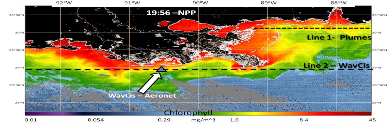
Figure 3. Location of east west transect (Line 2) which crosses the AREONET Wave_CIS Site. Clear waters in the east crossing the southwest pass of Mississippi river discharge.
