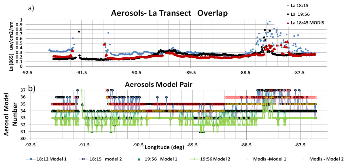
Figure 7. a) Aerosol radiance at 865 nm ( L_a ) across the transect is similar. Slight increase in the 18:15(blue) than for 19:55 or MODIS. b) Aerosol model pair used for epsilon selection of epsilon were similar: 18:15 used models 35-36, 34-35, 19:55 used 32-33 and 33-34 and MODIS used 35-36.
