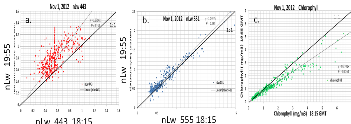
Figure 5. Differences are shown in scatterplot of a) nLw 443 b) nLw 555 and c) Chlorophyll along the transect between 18:15 and 19:55 GMT orbits.
