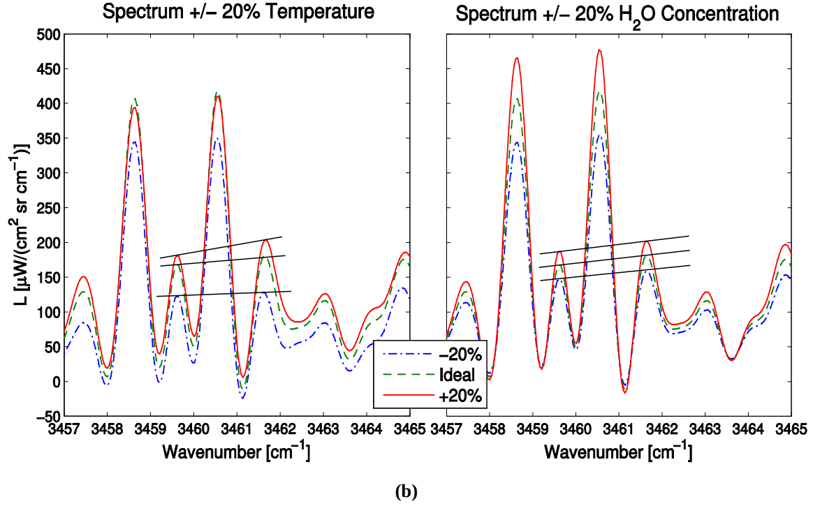
Figure 11: (a) Generated spectrum and CO 2 contribution for ideal \Phi = 0.91 flame at equilibrium. (b) Comparison of model generated spectrum for ideal flame to generated spectra at \pm 20\% temperature and H 2 O concentration. Temperature increase does not raise line shapes linearly because its relation to the model is exponential. H 2 O concentration increase raises line shapes linearly.
