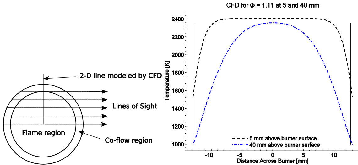
Figure 32: (left) Top view representation of how IFTS instrument “sees” flame vs. 2-D CFD approximation. (right) CFD plot of T vs radius at 5 and 40 mm above burner surface.
