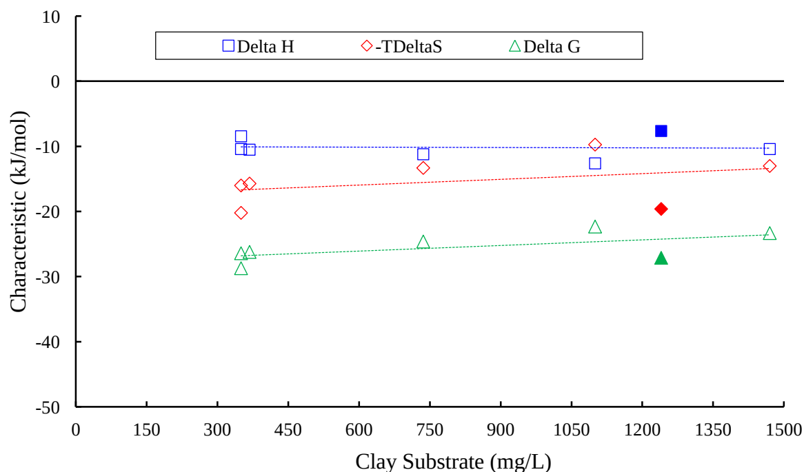
Figure 12. Thermodynamic profile as a function of clay concentration. Suspengel 200 (open symbols) and Aldrich K10 (filled symbols) data are shown. Reactions were conducted at 298 K. In all cases, the slopes of the linear regression lines were not significantly ( P = 0.05 ) different from zero.
