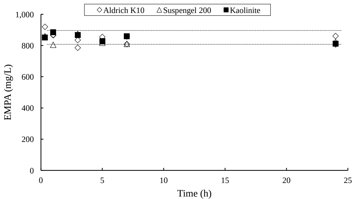
Figure 28. Initial kinetic sorption profiles for phosphonic acid degradation products. Top : MPA; bottom : EMPA. Dashed lines indicate the estimated 95% confidence intervals for the control (no substrate) samples. Profiles were obtained at 298 K, and all samples were filtered.
