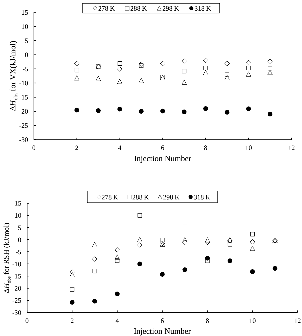
Figure 27. Injection-to-injection repeatability during pseudo-first-order reactions. Top: VX; bottom: RSH. In both cases, the substrate was Suspensgel 200.
