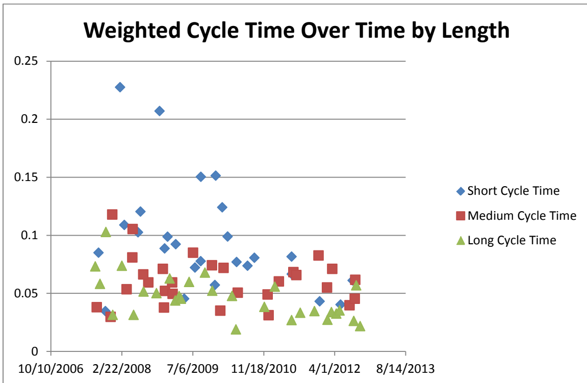
Figure 13. Availability Weighted Cycle Time Over Time by Defined Length
