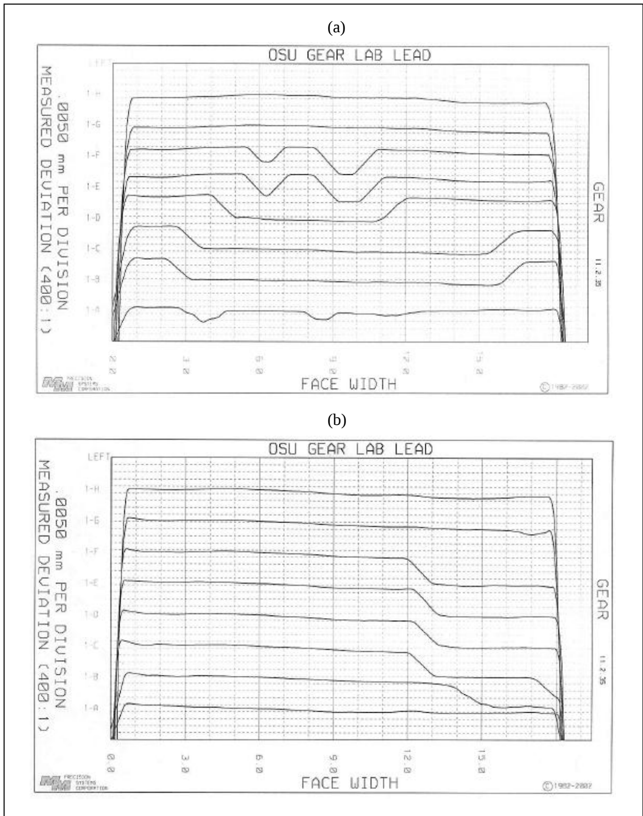
Figure 40. CMM lead traces of NiB-coated teeth after completion of efficiency test: (a) NiB-coated gear (not heat treated) and (b) NiB-coated gear (heat treated).
