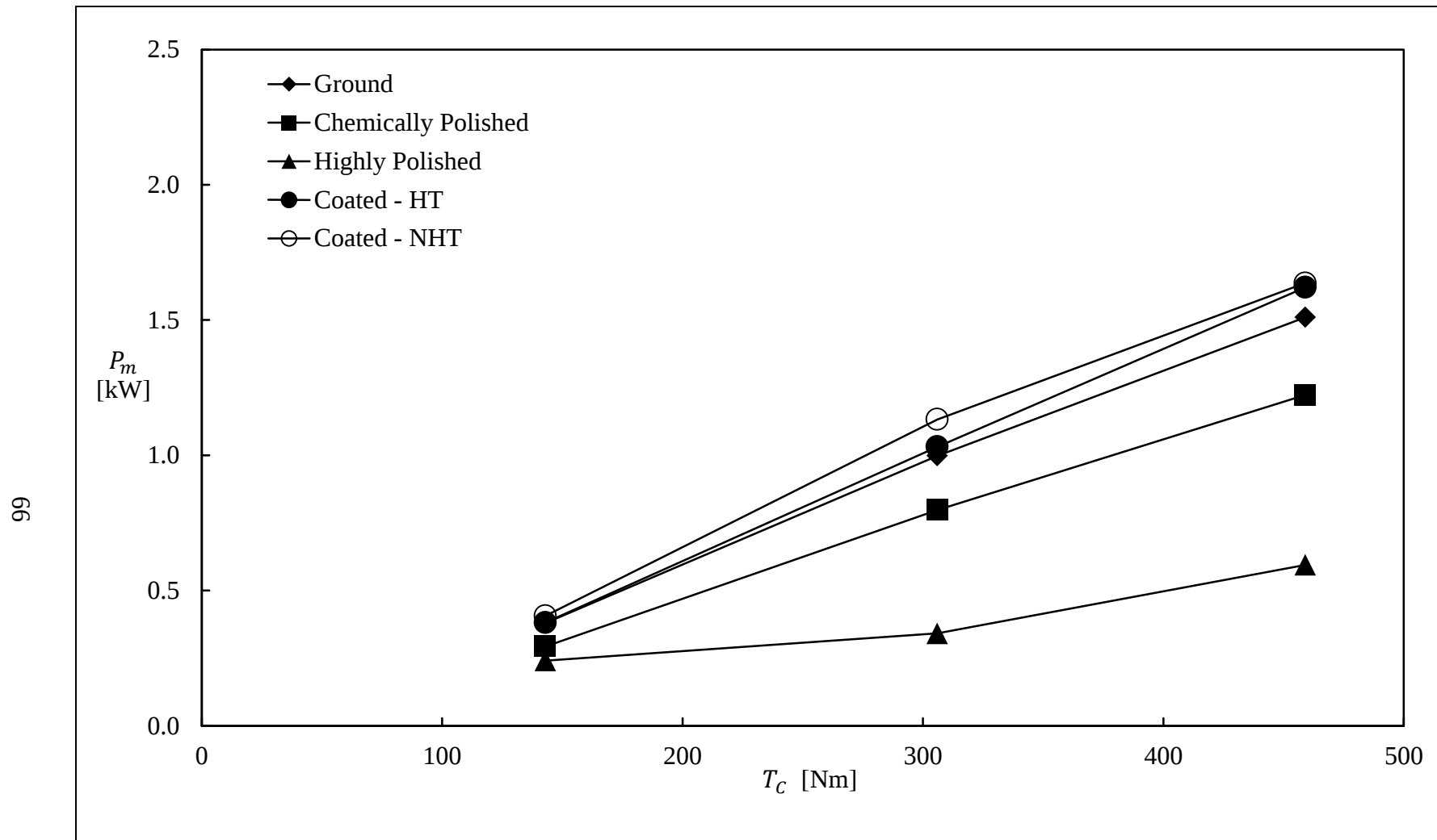
Figure 46. Comparison of measured mechanical power losses of gear pairs having different surface treatments at \Omega = 4000 rpm.
