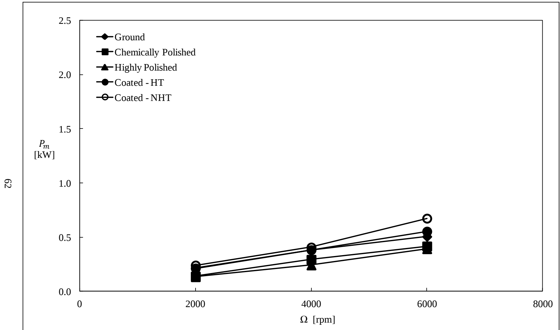
Figure 42. Comparison of measured mechanical power losses of gear pairs having different surface treatments at T_c = 143 Nm.
