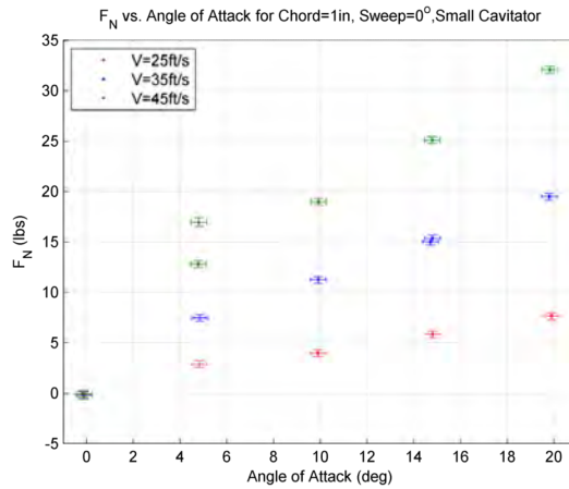
Figure D.25: Normal Force F_N vs. Angle of Attack and Tunnel Velocity, 1 inch chord, \gamma = 0^\circ , small cavitator
