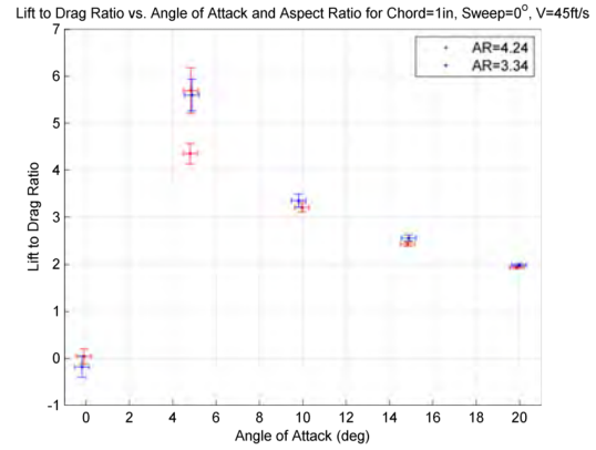
Figure 4.47: Lift/Drag Ratio from the unswept fin testing plotted against angle of attack and aspect ratio, 1 inch chord, R_n = 4.0 \times 10^5 , F_r = 27.5
