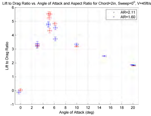
Figure 4.46: Lift/Drag Ratio from the unswept fin testing plotted against angle of attack and aspect ratio, 2 inch chord, R_n = 8.1 \times 10^5 , F_r = 19.4
