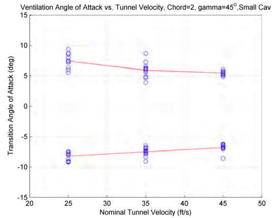
Figure E.10: Angle of attack where fin transitioned to fully ventilated, 2 inch chord, \gamma = 45^\circ , small cavitator
