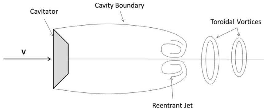
Figure 1.3: Reentrant Jet Cavity Closure Showing Ventilation Gas Expulsion through Toroidal Vortices
