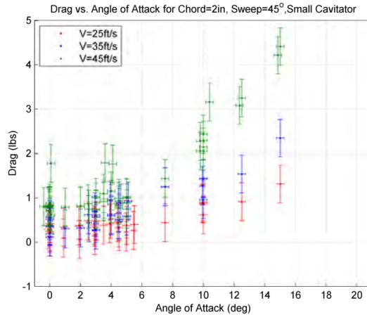
Figure D.23: Drag vs. Angle of Attack and Tunnel Velocity, 2 inch chord, \gamma = 45^\circ , small cavitator
