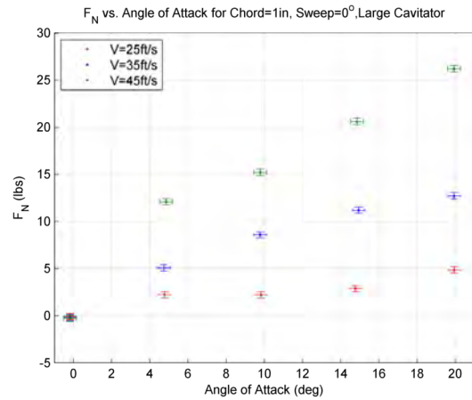
Figure D.26: Normal Force F_N vs. Angle of Attack and Tunnel Velocity, 1 inch chord, \gamma = 0^\circ , large cavitator
