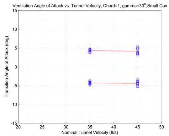
Figure E.6: Angle of attack where fin transitioned to fully ventilated, 1 inch chord, \gamma = 30^\circ , small cavitator
