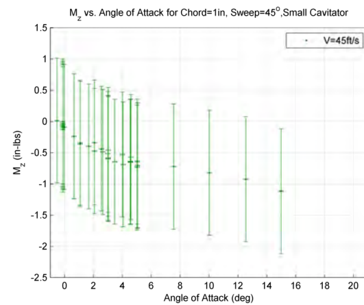
Figure D.58: Shaft Torque M_z vs. Angle of Attack and Tunnel Velocity, 1 inch chord, \gamma = 45^\circ , small cavitator
