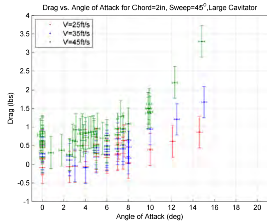
Figure D.24: Drag vs. Angle of Attack and Tunnel Velocity, 2 inch chord, \gamma = 45^\circ , large cavitator
