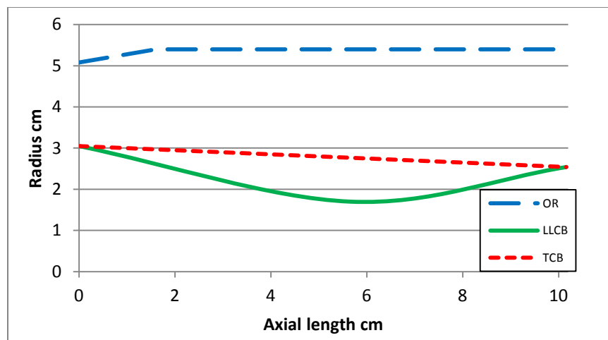
Figure 42. Radius distributions for LLCB and TCB designs
