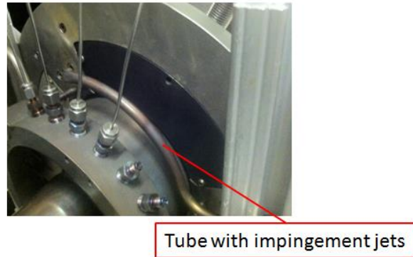
Figure 50. Impingement cooling air array (1 of 3)
