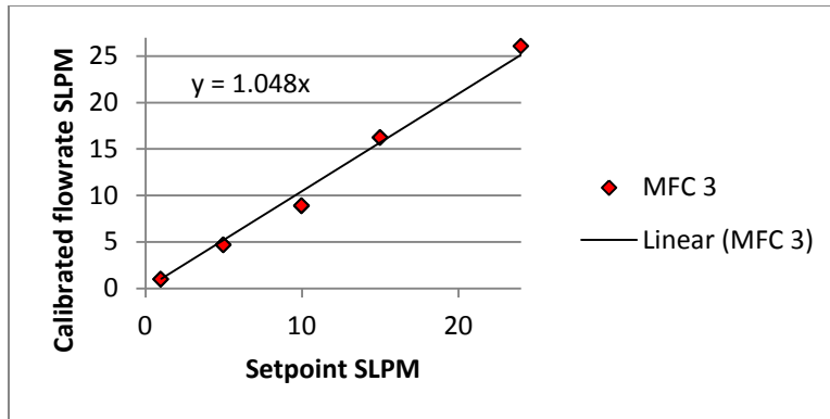
Figure 91. MFC 3 Calibration
