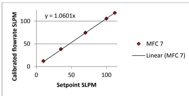
Figure 95. MFC 7 Calibration
