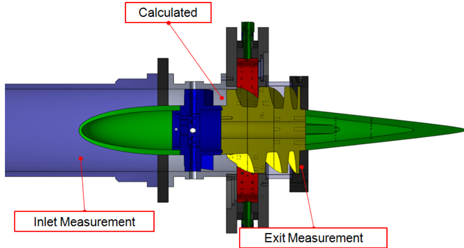
Figure 61. Total and static pressure and temperature probe locations for Rayleigh loss study
