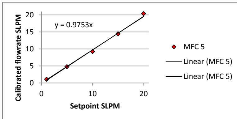
Figure 93. MFC 5 Calibration
