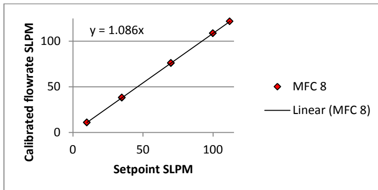
Figure 96. MFC 8 Calibration
