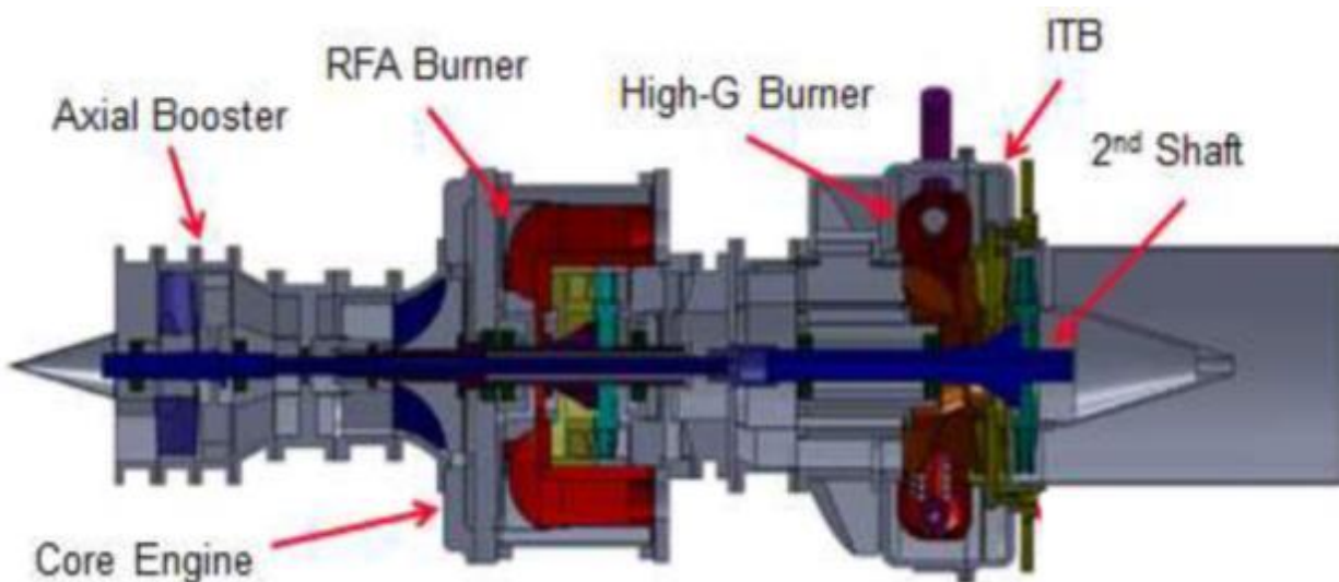
Figure 19. Spytek JI-304 outfitted with UCC ITB system to drive an axial boost stage [23]
