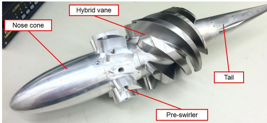
Figure 46. Full center section of the UCC
