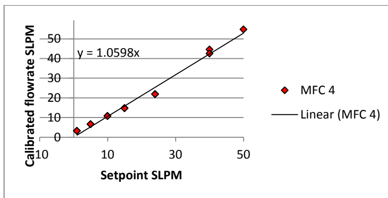
Figure 92. MFC 4 Calibration
