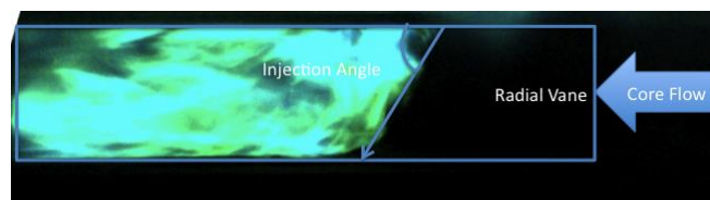
Figure 24. High speed video image of cavity migration angle into the core stream [20]
