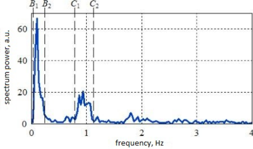
Figure 2.3: A continuation of Kamshilin's work, this is the power spectrum resulting from the fast Fourier transform applied to the type of data shown in Fig 2.2. Two prominent spikes are indicated in the graph, the first one at approximately 0.13Hz, which corresponds to the respiration rate, and the second at approximately 1.0Hz, which corresponds to the heartbeat rate. The researchers select and use these two narrow bands, B_1 - B_2 and C_1 - C_2 , as reference functions for the breathing cycle, and the cardiac cycle, respectively [2].
