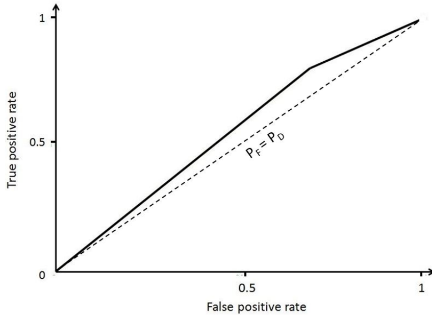
Figure 4.8: ROC curve for the most successful validation result among the Combo validation sets, which results from NASAIDS-IDF1 features and a decision tree classifier. The Combo dataset is validated with data collected with a NC fore optic. The set is comprised of 112 samples of “stress” and “non-stress” and six features.
