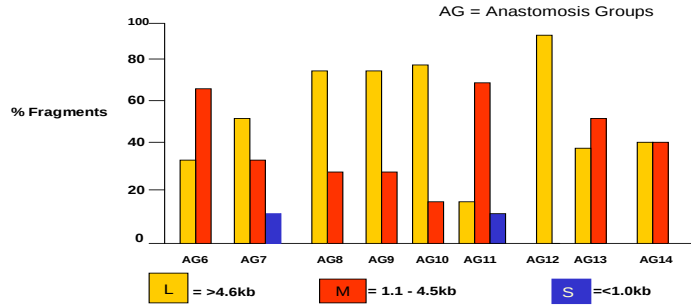
Figure 7: Size distribution profiling of dsRNA from viruses infecting different R. solani isolates. The dsRNA could be broadly classified into Large (L) (>4.6 kilo-bases); Medium (1.1-4.5 kilo-bases); and Small (<1.0 kilo-bases).
