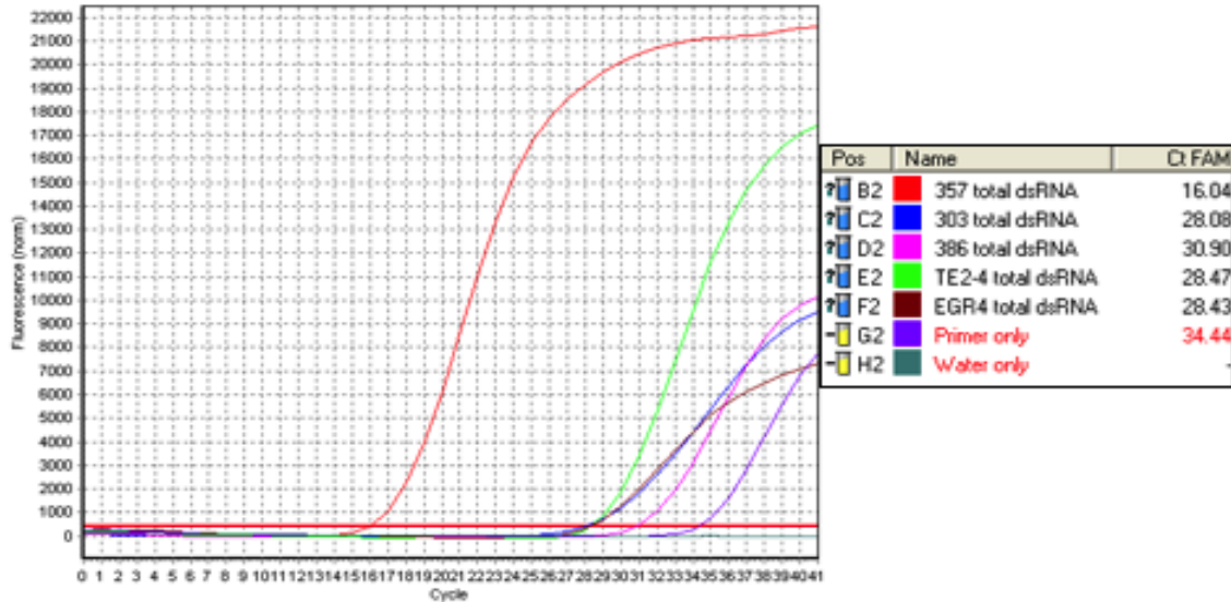
Figure 17: Real-Time PCR analysis using primers specifically obtained from the isolate 357 and probes designed from 357.
