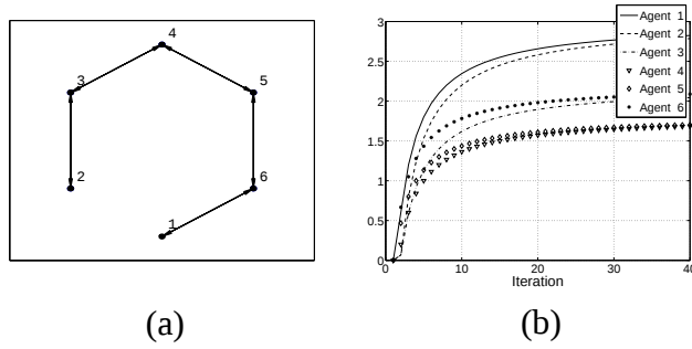
Fig. 5. A typical response of adaptive play, with M = 2 and p = 0.1 , under \kappa_0 = 1/4 and \kappa_1 = 0 : (a) Final graph, (b) Running average of mean distance from neighbors with time.
