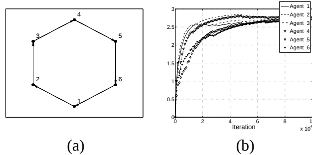
Fig. 7. A typical response of state-based reinforcement learning (11) with \lambda = 0.01 and \nu = 2/3 , under \mathfrak{C} with \kappa_0 = 1/4 , \kappa_1 = -1/10 : (a) Final graph, (b) Running average of mean distance from neighbors with time.
