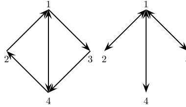
Fig. 2. Two Nash networks for n = 4 agents under \mathcal{C} with \delta - \delta^2 \leq \kappa_0 < \delta - \delta^3 and \kappa_1 = 0 .
