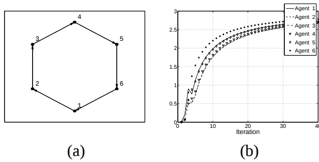
Fig. 6. A typical response of adaptive play, with M = 2 and p = 0.1 , under \mathfrak{C} with \kappa_0 = 1/4 and \kappa_1 = -1/10 : (a) Final graph, (b) Running average of mean distance from neighbors with time.
