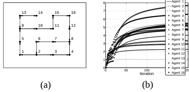
Fig. 3. A typical response of adaptive play, with M = 2 and p = 0.1 , under \mathfrak{C} with \kappa_0 = 1/8 and \kappa_1 = 0 : (a) Final graph, (b) Running average of mean distance from neighbors with time.
