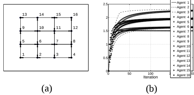
Fig. 4. A typical response of adaptive play, with M = 2 and p = 0.1 , under \mathfrak{L} with K = 3 , \kappa_0 = 1/8 , \kappa_1 = 0 and \gamma = 1/2 : (a) Final graph, (b) Running average of mean distance from neighbors with time.
