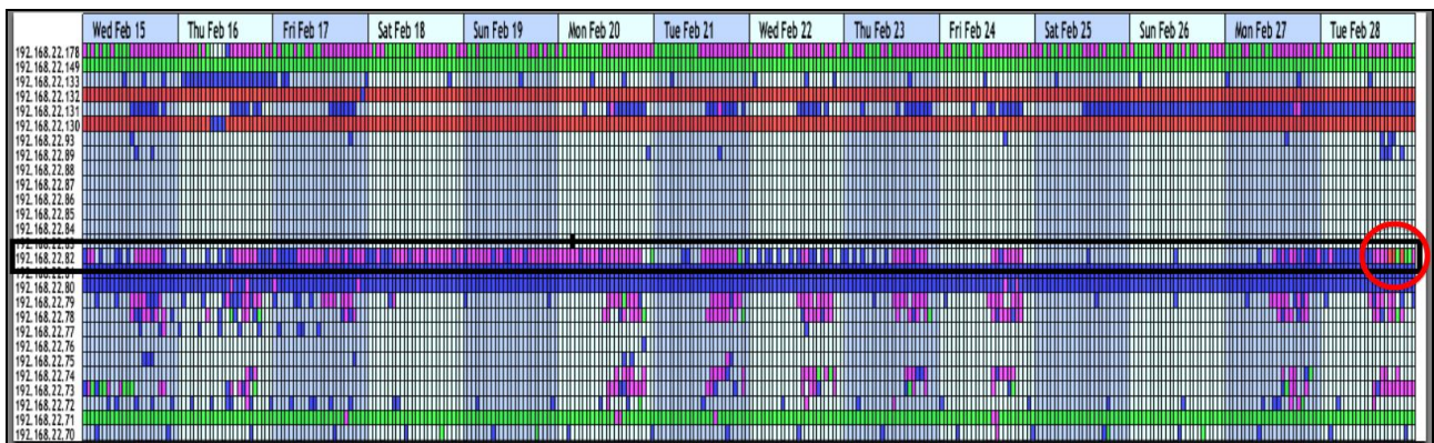
Figure 4: Discovering a change in the pattern of behavior
