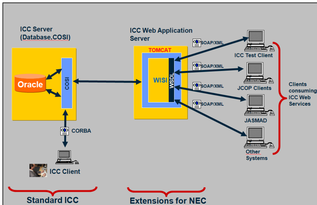
Figure 3. ICC Web Service Architecture
