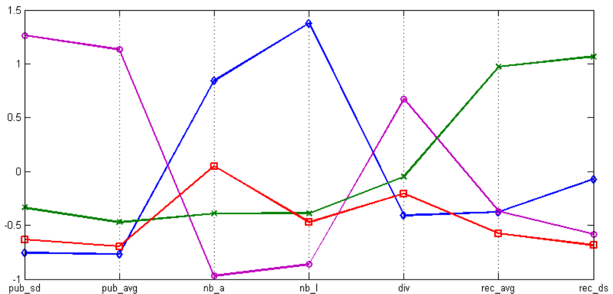
Figure 3: Centroids visualization on parallel coordinates
