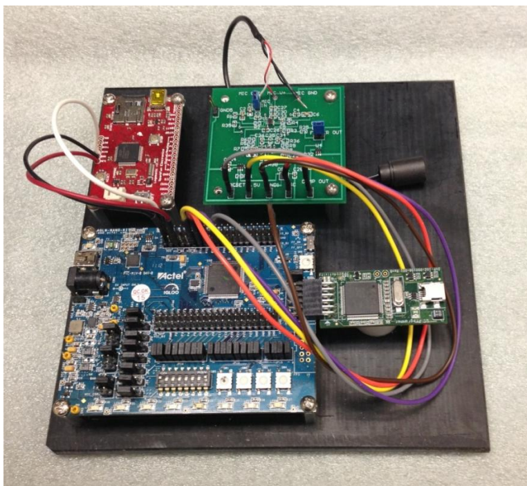
Figure 10. LPAD breadboard.
