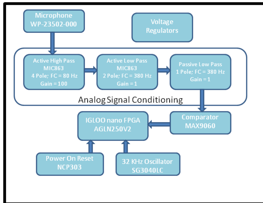
Figure 3. LPAD block diagram.
