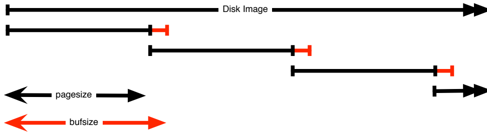
Figure 16: Image Processor divides the disk image into buffers. Each buffer is the size of a page ( pagesize ) with a buffer overlap in an area called the margin. ( marginsize is equal to bufsize-pagesize ). The buffers overlap with each other to ensure all information is processed.
