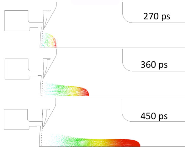
Fig. 16. Beginning stages of bunch formation.
