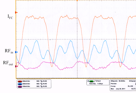
Fig. 4. Measured Faraday cup current, I_{FC} , for combined first and third harmonic modulation of the electron gun. The parameters are V_{cathode}=-36 kV, V_{grid}=-90 V, with \sim 540 W at 714 MHz and \sim 450 W at 2142 MHz. The microbunches are 325 ps FWHM (135 ps RMS), with 2.81 A peak current and \sim 0.91 nC per bunch. Also shown are RF_{in} and RF_{out} .
