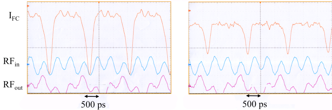
Fig. 6. Faraday cup data for combined first and third harmonic modulation of the electron gun and higher negative grid bias for V_{\text{cathode}}=-36 kV and \sim 200 W at 714 MHz and \sim 450 W at 2142 MHz. The left traces correspond to V_{\text{grid}}=-100 V; the right traces correspond to V_{\text{grid}}=-125 V.
