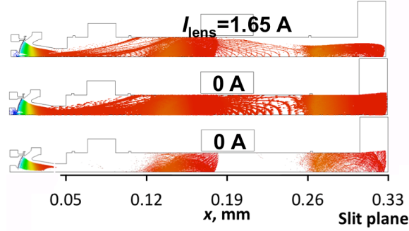
Fig. 10. Simulation of the emission measurements at V_{\text{cathode}} = -32 kV and effect of the emission from the central hole. Electron trajectories for: (top) I_{\text{lens}} = 1.65 A and (center) I_{\text{lens}} = 0 A include emission from the central hole; (bottom) I_{\text{lens}} = 0 A is with emission from the central hole suppressed.
