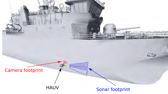
(b) The HAUV inspecting a ship hull
