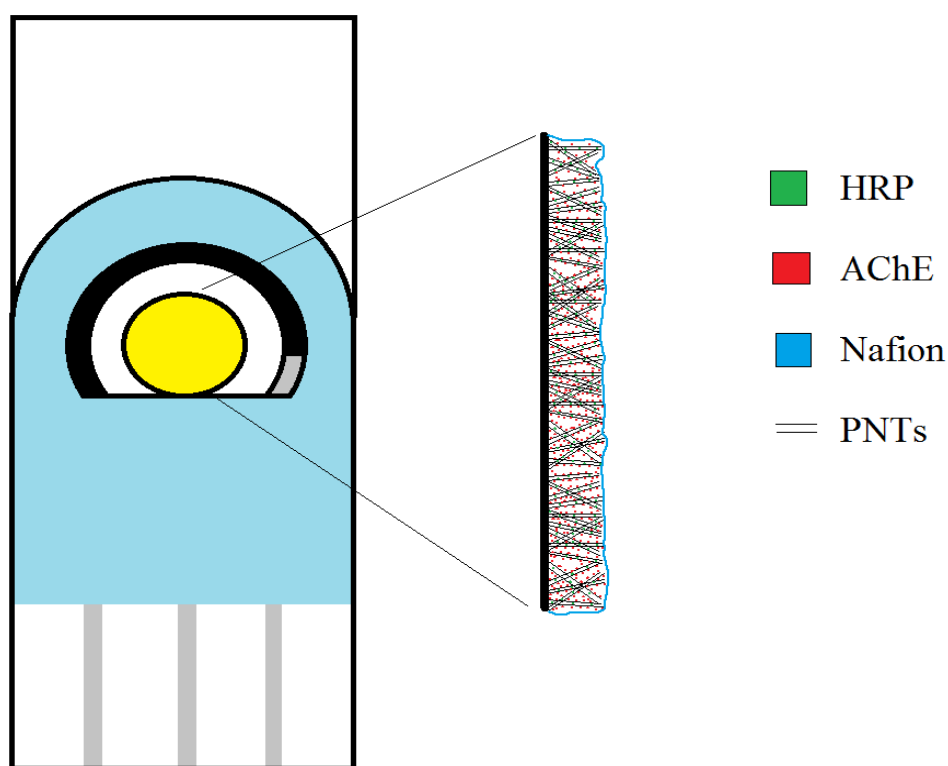
Figure 4. Electrode Construction
