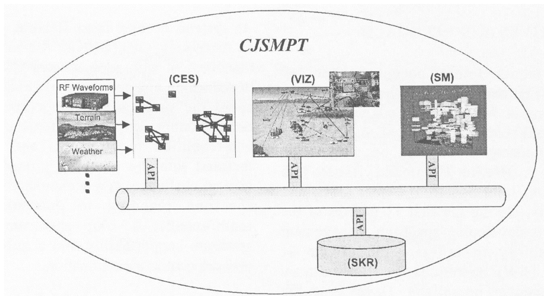
Figure 3: CJSMP Architecture.
