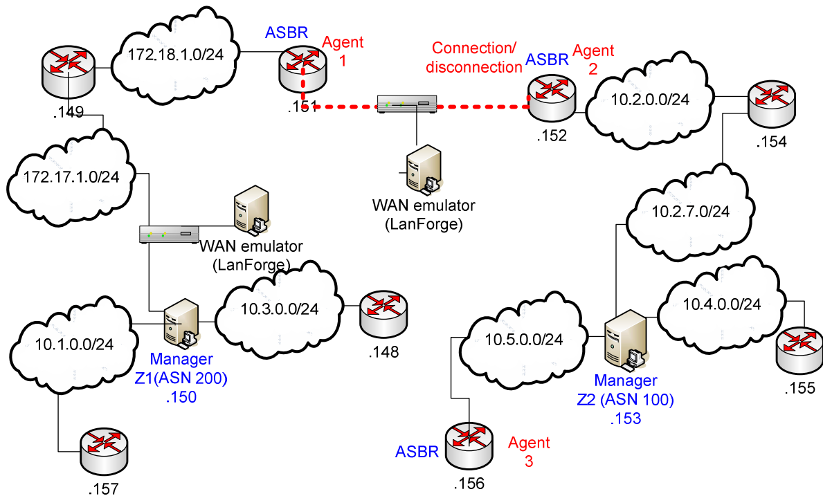
Figure 11: Testbed for validation tests
