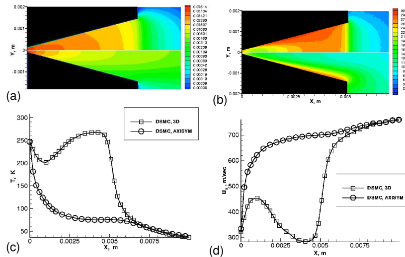
Figure 4: Cold gas thruster results. Portions (a) and (b) show a comparison of the flows for a 3-D (top) and a 2-D (bottom) geometry for gas density ( \text{kg/m}^3 ) and temperature (K), respectively. Portions (c) and (d) show a comparison of the temperature profiles and stream wise velocity, respectively, along the nozzle axis from the throat to a region downstream of the exit for the 3-D versus an axisymmetric geometry.
