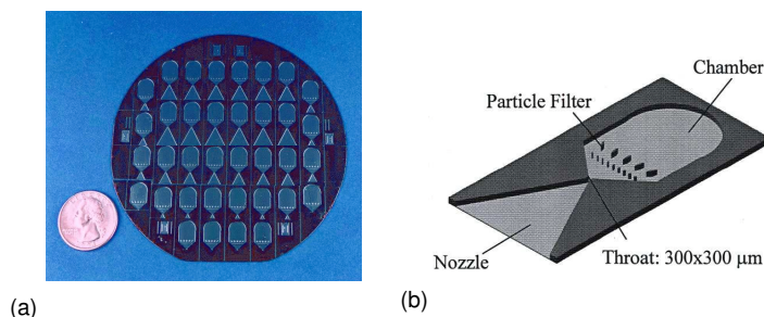
Figure 2: MEMS fabrication concept of an array (a) and a single (b) thruster.(22)
