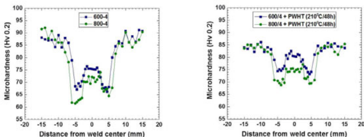
Fig. 4. Microhardness data for as processed and PWHT samples.
