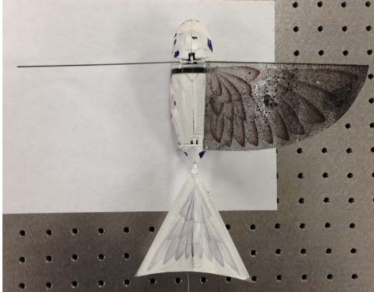
Figure 17. Top view of the test article used for modal testing with the wing membrane removed from the leading edge beam on the left side. This configuration would show different results than the bar in the clamped configuration.
