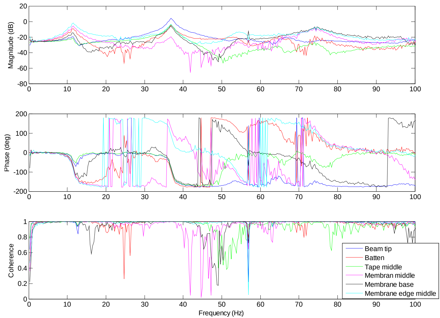
Figure 34. FRF and coherence for wing in clamped configuration at six different points.
