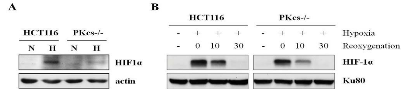
Exp 1: A: Westernblot analysis of HCT116 WT and DN-PKcs null cells. Cells were incubated in normoxia (N) and hypoxia (H) for 4 hrs followed by lysis. Whole cell lysates were then subjected to Westernblot analysis for HIF-1 \alpha and actin. B: HCT116 and DNA-PKcs -/- cells were subjected to 4 hrs of hypoxia followed by reoxygenation for indicated times and then subjected to WB analysis for HIF-1 \alpha and and Ku80
