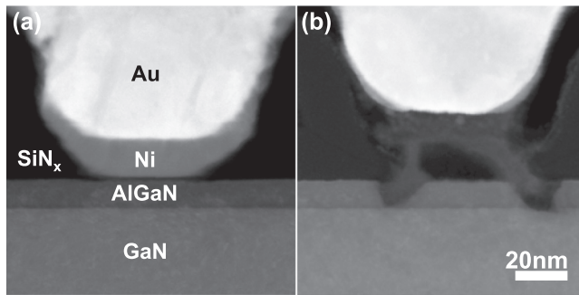
FIG. 3. High magnification HAADF-STEM images of the gate region of AlGaIn/GaN HEMTs showing the distinct gate metal stack layers and semi-conducting epilayers in (a) devices experiencing “slow” degradation, which are basically indistinguishable from unstressed devices and (b) in devices experiencing “rapid” degradation showing an “arch”-shaped defect formed from the original Ni layer of the gate and penetrating into the AlGaIn epilayer.
