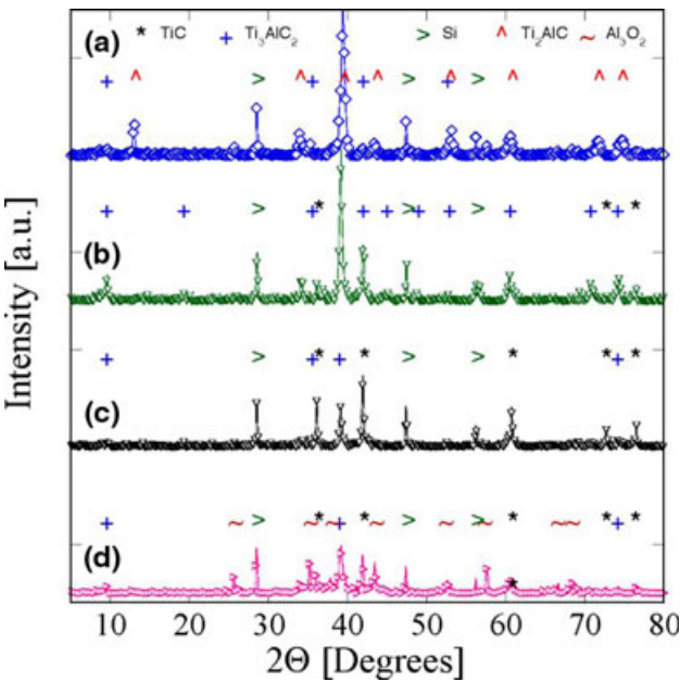
Fig. 4. X-Ray diffraction spectra of samples, (a) 10-17-HIP-1300, (b) 10-9-HIP-1500, (c) 3-9-HIP-1500, and (d) 10-46-HIP-1500. All spectra normalized to 10 wt% Si.
