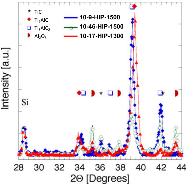
Fig. 5. X-ray diffraction spectra from 28 to 44° 2θ of samples 10-9-HIP-1500, 10-46-HIP-1500, and 10-17-HIP-1300.
