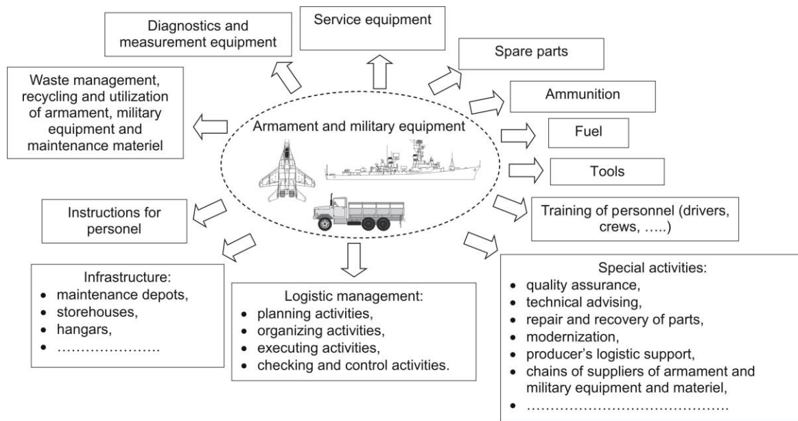
Fig.9. Logistic requirements of armament and military equipment
