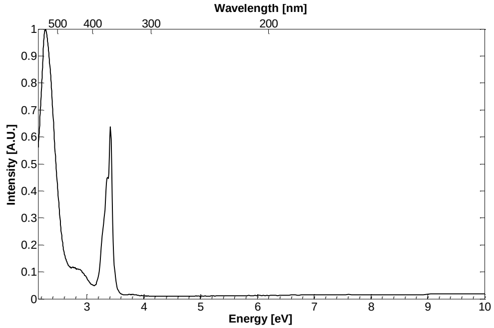
Figure C-2: Data taken on a crystalline GaN sample. A peak was observed at 363 nm (3.41 eV), which exactly matches the experimentally measured band gap of GaN at room temperature. [33]
