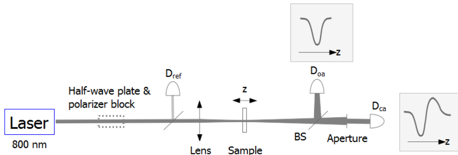
Fig. B1. Z-scan setup schematics. Here D_{oa} , D_{ca} , and D_{ref} are the opened-aperture, closed-aperture, and reference detectors, respectively, BS is the beam splitter, the focal length of the lens is 400 mm.
