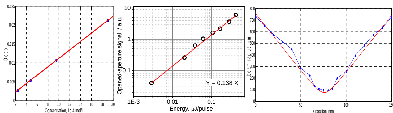
Fig. B4. (A) Dependence of the z-scan amplitude (deep) at the minimum as a function of the sample concentration (0.3 \mu\text{J}/\text{pulse} laser power). (B) Z-scan amplitude at the focus as a function of laser power. Both dependencies were measured for the [\text{Ru}(\text{pyr-v-ph-bpy})_2(\text{en})][\text{PF}_6]_2 complex. (C) Laser beam profile.
