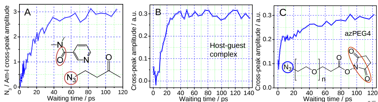
Fig. E2. Waiting-time \text{N}_3 /amide-I or \text{N}_3 /C=O cross-peak dependencies (A) for a 1:1 mixture of compounds shown in the inset, (B) for a 1:1 host-guest complex (see text), and (C) for azPEG4, all in chloroform.
