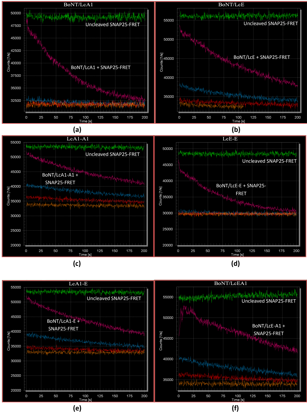
Figure 1: Förster Resonance Energy Transfer (FRET) based analysis of enzymatic activity of BoNT/LCs. Time-based cleavage of SNAP25-FRET substrate by (a) BoNT/LcA1 (b) BoNT/LcE (c) BoNT/LcA1-A1 (d) BoNT/LcE-E (e) BoNT/LcA1-E and (f) BoNT/LcE-A1. The magenta line shows the first 200 seconds of activity, blue line shows 200-400 seconds, red line 400-600 seconds and the orange line shows the final 600-800 seconds of activity.
