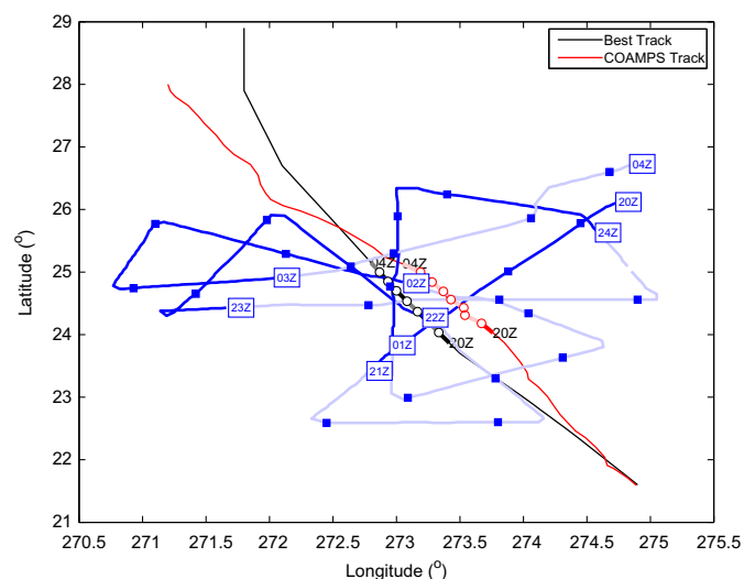
Fig. 8. Flight track of the airborne SRA (blue line) starting at 2000 UTC 14 September 2004 and ending at 0400 UTC 15 September 2004. Full hours are printed in boxes and 15 min intervals are denoted with blue squares. Flight segments starting with even (odd) hours are colored dark (light) blue. The observed (black) and simulated (red) TC tracks are shown. The circles on the two tracks represent hourly locations of the storm center.
