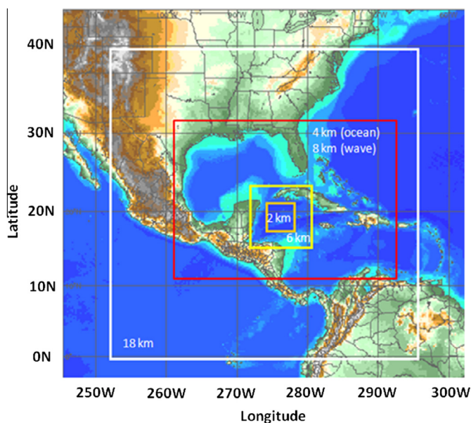
Fig. 2. Atmospheric 18-km (white), 6-km (yellow), and 2-km (orange) resolution grids and ocean/wave 4/8-km (red) resolution grids used for Hurricane Ivan simulations. The two inner atmospheric grids move in tandem with the center of the TC. The domain of the ocean and wave grids is large to allow for appropriate numerical spin-up of the cyclone over the Caribbean Sea before entering the Gulf of Mexico.
